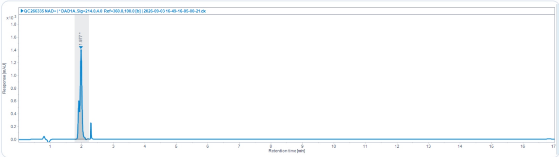
HPLC Chromatogram · Retention Time 1.977 min
