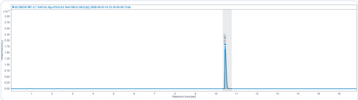
HPLC Chromatogram · Retention Time 10.442 min
